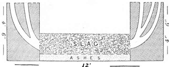
BLAST FURNACE FOUND IN MOUND AT LACHISH. (See p. 418.)
