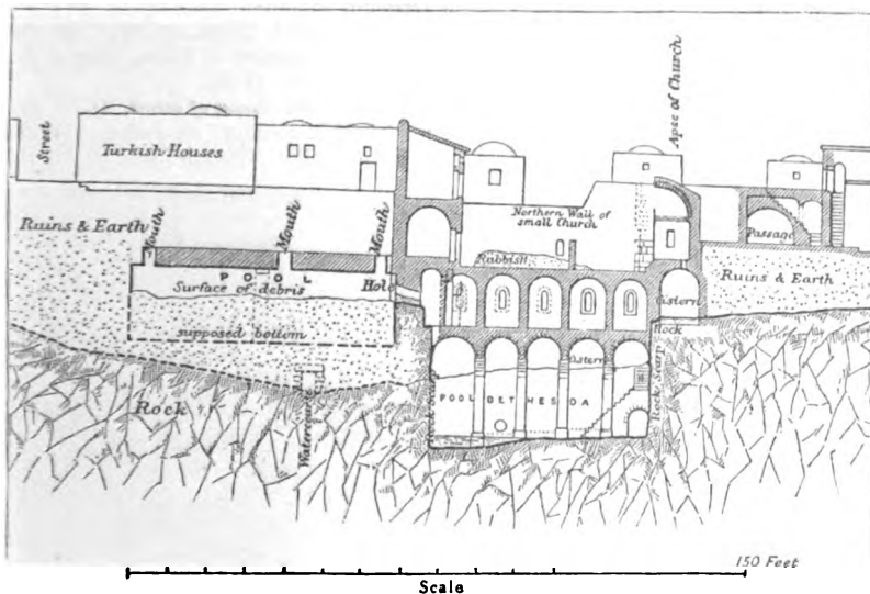
PROBABLE POOL OF BETHSADA. SECTION FROM EAST TO WEST. (By permission of the Committee of the Palestine Exploration Fund.)
